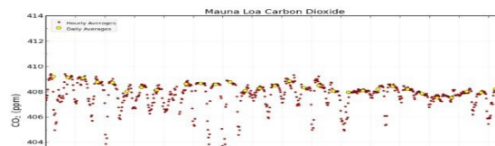
Recent Daily Average Mauna Loa CO 2
