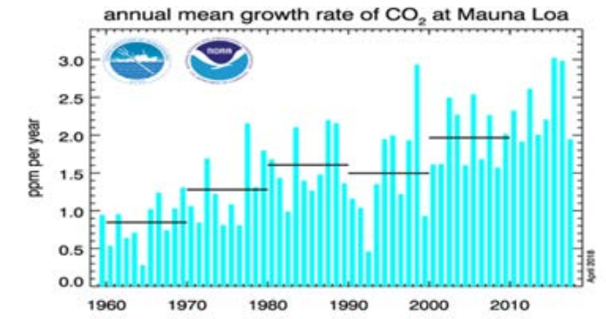
Graph 6: Mauna Loa CO 2 Rate of Rise [16].
