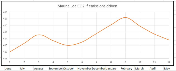
Graph 8: Mauna Loa if emissions driven (calculated) (D. White 2020).
