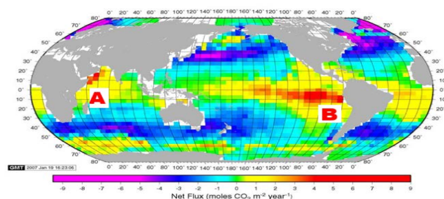
Figure 6: Takahashi 1997 Ocean Surface CO 2 [21].
