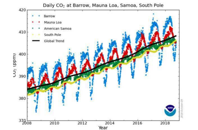
Graph 5: Mauna Loa cycles [16].
