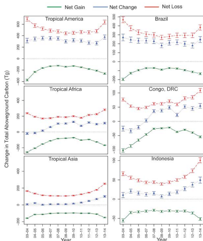
Figure 1: Figure 1: Most southern hemisphere tropical forests have switched to be an oxygen sink and carbon dioxide producer. Annual net change (95% confidence interval) in total carbon. Red lines indicate a loss in carbon; green lines indicate a gain. Blue lines reflect the difference between losses and gains. The vertical bars indicate the standard error of the change value [11].
